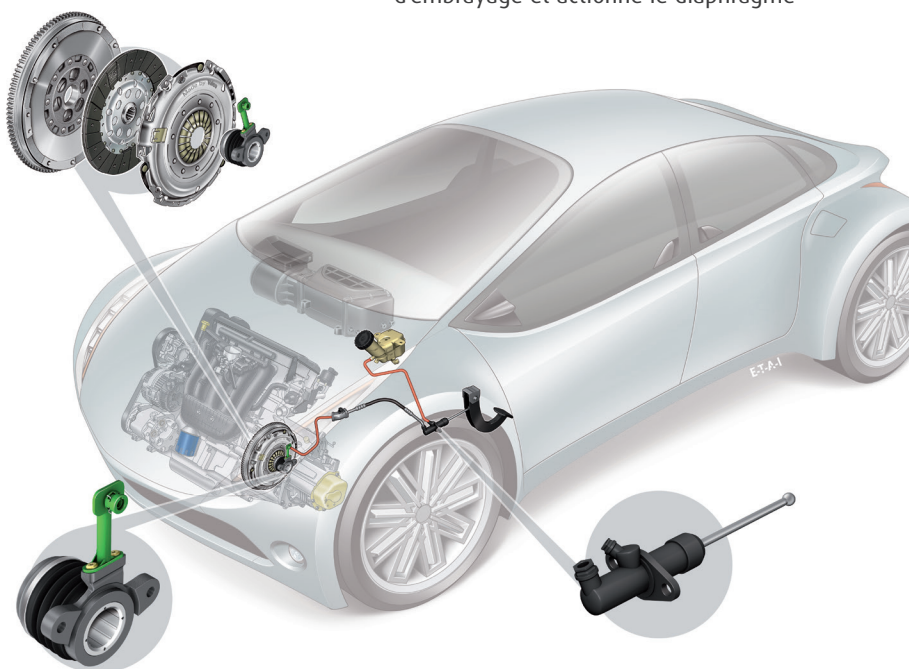
*CMC : clutch master cylinder / CRC : clutch release cylinder / CSC : concentric slave cylinder
